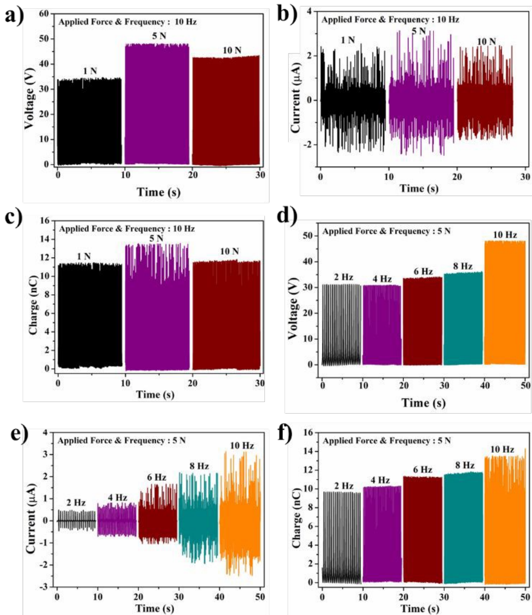
Figure 6. Triboelectric output on varying the force a) V_{oc} b) I_{sc} and c) transferred charge
