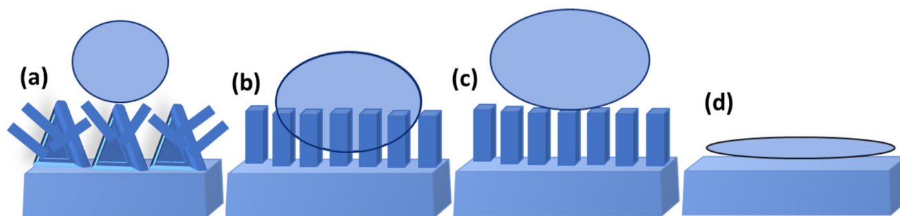
Fig. 6 Illustration of the behaviour of water droplets based on the (a) Lotus effect, (b) Wenzel model, (c) CB (Cassie–Baxter) model, and (d) superhydrophilic behavior. 11,15
