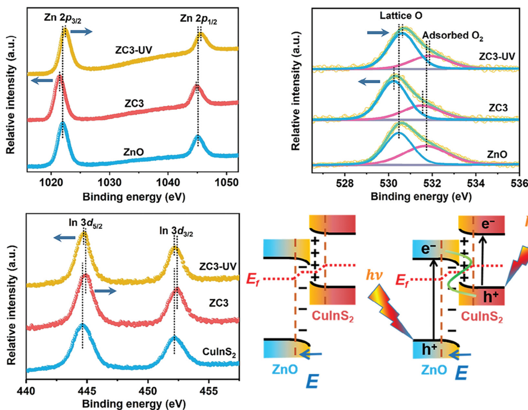
Fig. 5 XPS spectra recorded in the dark and under UV light from a 365 nm LED. The proposed interfacial electron transfer is also schematically illustrated. Reprinted with permission from ref. 25. Copyright 2024, Wiley-VCH GmbH.
