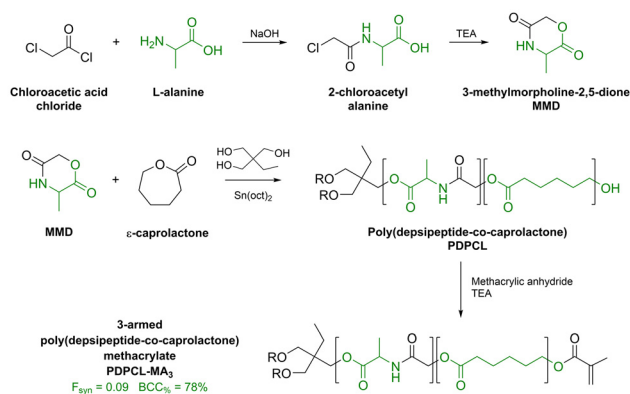
Scheme 11 Synthesis of photocurable PDPCL-MA3. The biobased portion of each structure is depicted in green. TEA = triethylamine, Sn(oct) 2 = tin(II) bis(2-ethylhexanoate). Re-drawn from ref. 172.
