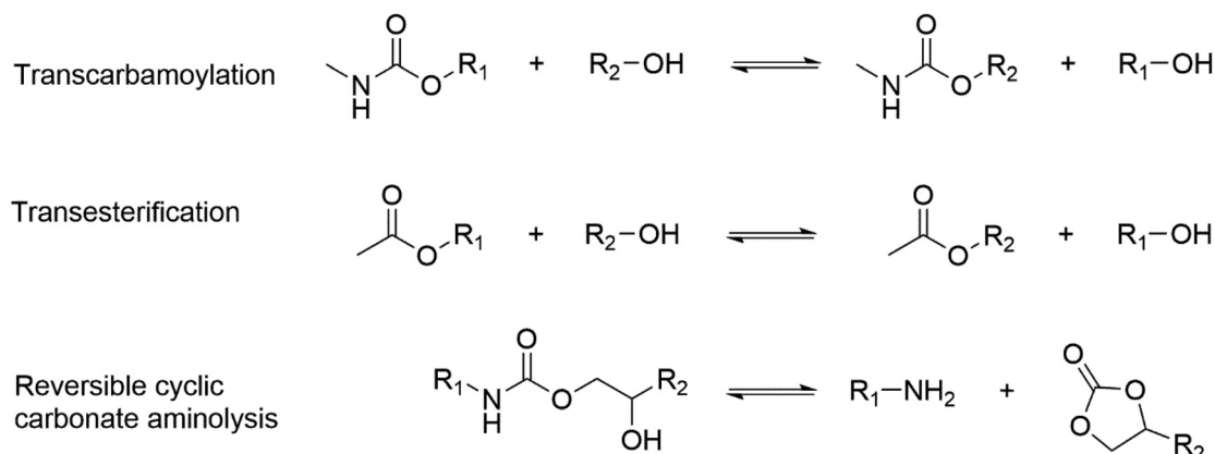
Scheme 13 Reversible cyclic carbonate aminolysis, transesterification and transcarbamylation reactions. 188
