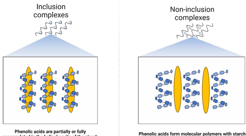
Fig. 3 Types of starch–phenolic acid complex.
