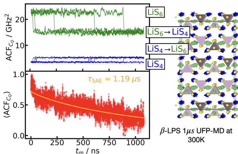
Fig. 5 \langle ACF_{C_0} \rangle for \beta -LPS. By considering only the Li atoms in the 300 K simulation which perform a hop to another site during the 1 \mu\text{s} simulation (either \text{LiS}_4 \rightarrow \text{LiS}_6 or \text{LiS}_6 \rightarrow \text{LiS}_4 ), and calculating the \langle ACF_{C_0} \rangle over these sites, we extract \tau of 1.19 \mu\text{s} . The colors of the individual atom ACF_{C_0} shown in the top left panel correspond to the starting site of the Li atom at time t = 0 . Thus \text{LiS}_6 sites at t = 0 which hop to \text{LiS}_4 sites have an ACF_{C_0} in green, and \text{LiS}_4 sites at t = 0 which hop to \text{LiS}_6 sites are shown in blue. The trajectories of all Li atoms are colored in the same fashion in the right panel of the Li atoms trajectory.
