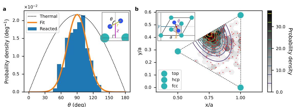
Figure 4: Distributions for initial (a) orientations \theta and (b) (x, y) positions of \text{N}_2 molecules above the Ru(0001) surface for E_{\text{inc}} = 3.25 \text{ eV} ( > E_{\text{a}}^{\text{TS}} = 1.83 \text{ eV} ) and \nu = 0 . The coordinates are depicted in the insets. a) The initial distribution for all trajectories (both reacted and non-reacted, black dashed line, Eq. S6 in the Supplementary Information) is compared to the distribution of the subset comprised by the reacted trajectories (blue bars). To guide the eye, the latter has been fitted to the initial distribution multiplied by a Gaussian centred at \theta = 90^\circ (orange line, Eq. S7 in the Supplementary Information). b) The distribution for the initial (x, y) -position of reacted trajectories in the irreducible wedge of the unit cell, as depicted in the inset. a denotes the surface lattice constant. Individual reacted trajectories are in red, the histogram is in greyscale, and the fitted bimodal Gaussian distribution are the contour lines. For better comparison and to quantify dynamical steering effects, the reacted distributions have been rescaled such that their maxima coincide with those of the distributions for all trajectories.
