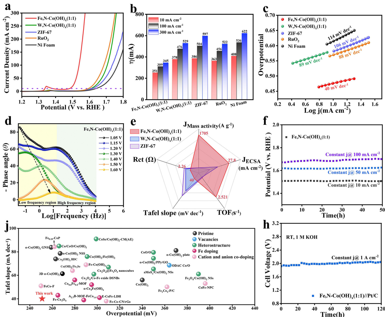
Fig. 3 Electrochemical performance and durability of Fe,N-Co(OH) x (1:1) for OER. (a) LSV polarization curves in 1 M KOH solution at a scan rate of 5 mV s -1 . (b) Overpotential ( \eta ) at 10, 100, and 300 mA cm -2 . (c) Tafel slopes for Fe,N-Co(OH) x (1:1) during the OER. (d) Bode plots for Fe,N-Co(OH) x (1:1) during the OER. (e) Comparison of OER activity between Fe,N-Co(OH) x (1:1) (red), W,N-Co(OH) x (1:1) (blue), and ZIF-67 (orange-red). (f) Chronopotentiometric curve at 10, 50, and 100 mA cm -2 . (g) Comparison with recently reported catalysts. (h) The long-term durability of the prepared AEMWEs (Fe,N-Co(OH) x (1:1)//Pt/C) measured at 1 A cm -2 current density (operated at room temperature at a flow rate of 0.15 L min -1 ).
