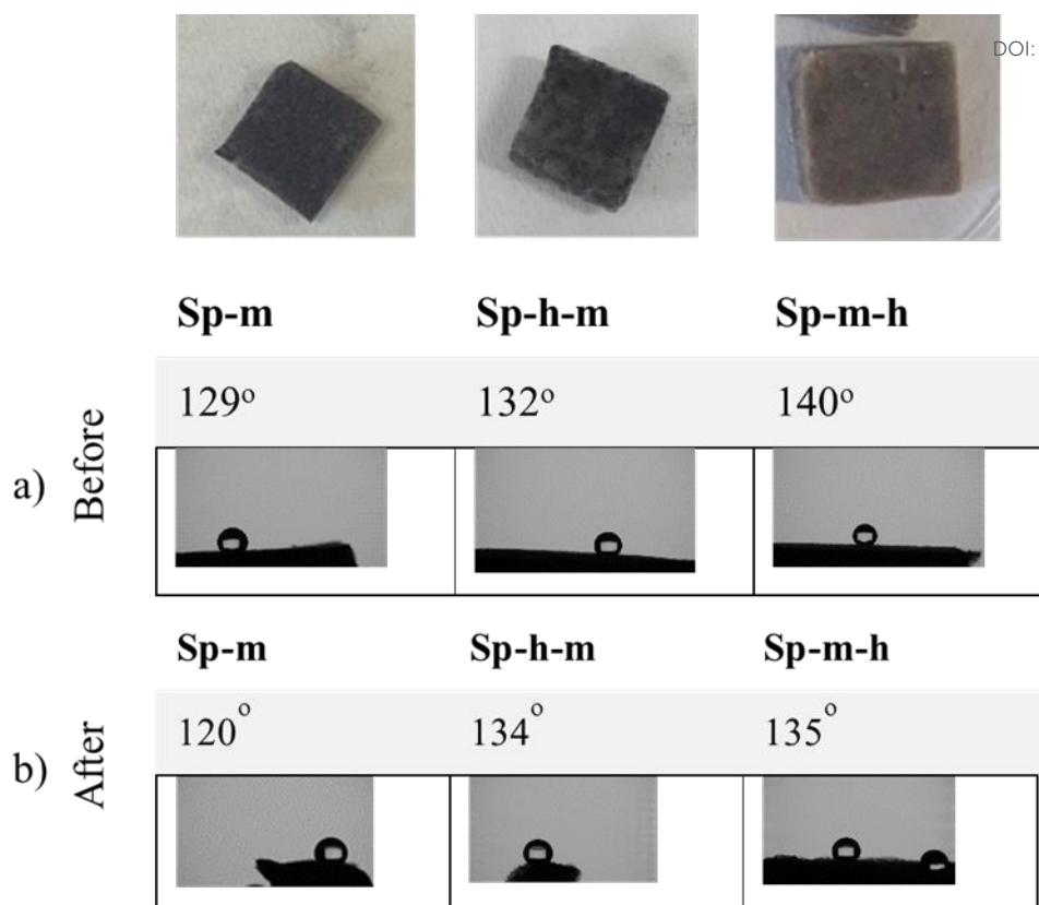
Figure 5. a) Photos of the Sp-m, Sp-h-m and Sp-m-h samples, as well as their initial contact angles with a droplet of water and b) the contact angles after the oil extraction and the subsequent purification process.
