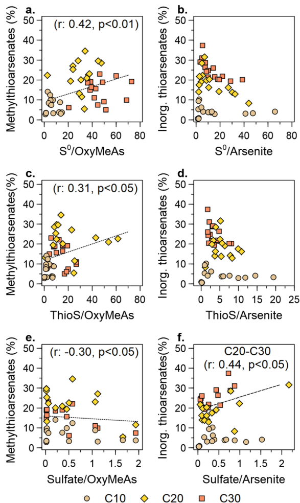
Fig. 5 Influence of excess S^0 , thiosulfate (ThioS), and sulfate over oxymethylated arsenates (OxyMeAs) in the formation of methylthioarsenates (a, c, and e, respectively). Influence of excess S^0 , thiosulfate (ThioS), and sulfate over arsenite in the formation of inorganic thioarsenates (b, d, and f, respectively).
