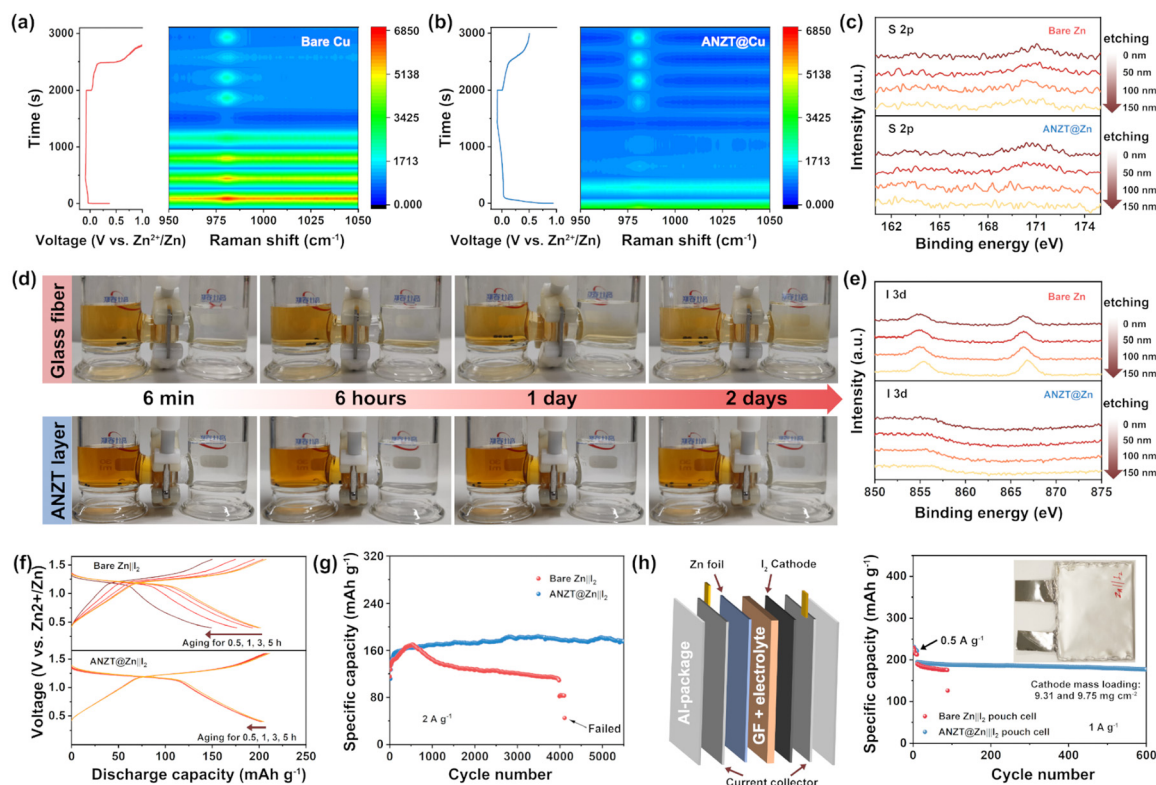
Fig. 5 In situ Raman spectra of (a) bare Cu mesh and (b) ANZT@Cu mesh during the Zn plating/stripping process. (c) The \text{Ar}^+ -etching high-resolution XPS spectra of S 2p of bare Zn and ANZT@Zn anodes after 50 cycles in the symmetric cells (at 5 \text{ mA cm}^{-2}/2.5 \text{ mA cm}^{-2} ). (d) Optical images of H-type glass mold with anolyte (left, 0.5 \text{ M KIO}_3 and 0.1 \text{ M I}_2 ), catholyte ( 0.5 \text{ M KIO}_3 ), and the GF separator with/without the ANZT coating layer. (e) The \text{Ar}^+ -etching high-resolution XPS spectra of I 3d of bare Zn and ANZT@Zn anodes after 100 cycles in the \text{Zn}||\text{I}_2 cells (at 1 \text{ A g}^{-1} ). (f) Electrochemical aging test (from 0.5 to 5 h standing after full charge state) for \text{Zn}||\text{I}_2 batteries with bare Zn (upper) and ANZT@Zn (lower) anodes. (g) The cycling performance of \text{Zn}||\text{I}_2 cells with bare Zn and ANZT@Zn anodes at a current density of 2 \text{ A g}^{-1} . (h) The cycling performance of \text{Zn}||\text{I}_2 pouch cells with different Zn anodes at a current density of 1 \text{ A g}^{-1} with the high cathode mass loading of 9.31 (bare Zn) and 9.75 (ANZT@Zn) \text{mg cm}^{-2} .
