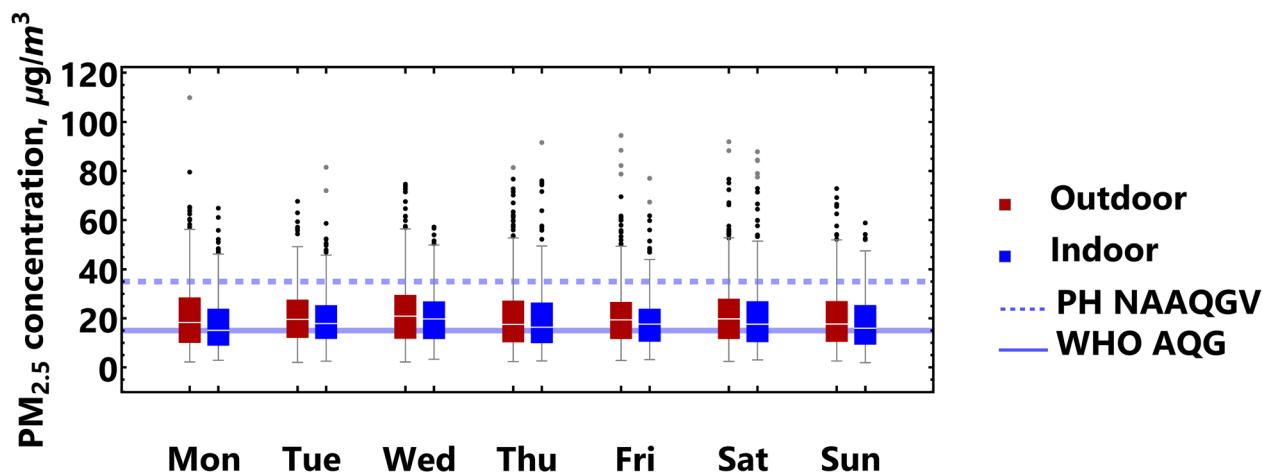
Fig. 3 Five-number summary (box-and-whisker) plots for day-of-the-week indoor and outdoor PM 2.5 . The solid horizontal blue gridline is the WHO AQG (15 μg m −3 PM 2.5 ) and the dashed blue horizontal line is the Philippine (PH) NAAQGV (35 μg m −3 PM 2.5 ), which were the applicable standards at the time of data collection. The black and gray points are outliers and far outliers, respectively.
