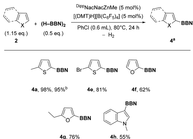
Chart 2 Substrate scope for zinc catalysed borylation. a Yield versus an internal standard. b Glove-box free procedure (see SI for details).
