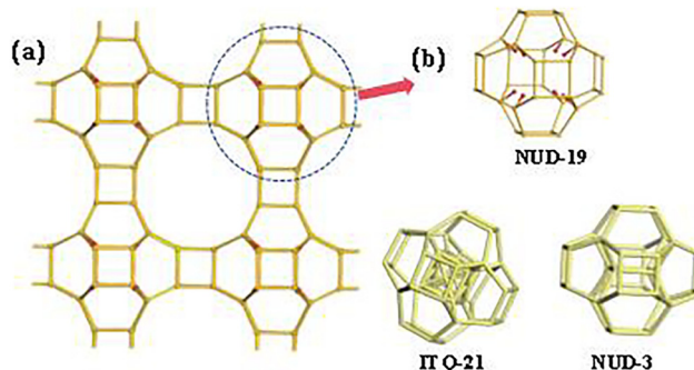
Fig. 4 Crystal structure (a) and structural unit (CBU) image (b) of NUD-19.
