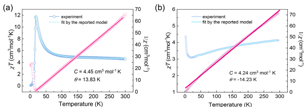
Fig. 3 Temperature dependence of \chi T values (blue circles) and 1/\chi (pink circles) measured from 2 to 300 K under a dc field of 1 kOe for 1 (a) and 2 (b). The solid red line represents the fitting based on the Curie–Weiss law. The solid sky blue line represents the fitting results based on the literature model. 40
