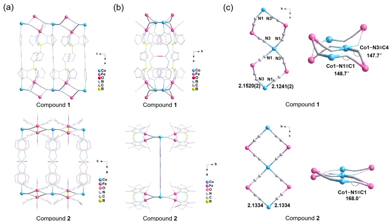
Fig. 2 Packing diagrams of compounds 1 and 2 in the ac -plane (a) and in the ab -plane (b). (c) The simple schematic of the side of two twisted \text{Fe}_2\text{Co}_2 square units of compounds 1 and 2. Hydrogen atoms and water molecules are omitted. Color code: Fe, pink; Co, sky blue; B, yellow; N, stone blue; C, gray purple; and O, red.
