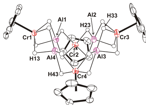
Fig. 5 Perspective view of 9 · 1.5C_7H_8 with thermal ellipsoids at the 50% probability level. Methyl groups of the \eta^5-C_5Me_5 ligands and toluene solvent molecules are omitted for clarity. Selected averaged lengths (Å) and angles ( ^\circ ): Cr–H 1.63(5) , Al–H 1.72(2) , Cr–Cm 1.808(2) , Cr–Al 2.376(2) , Cr(1)/Cr(3)···Cr(2) 4.748(2) , Cr(1)/Cr(3)···Cr(4) 4.750(4) , Cr(2)···Cr(4) 6.119(1) , Cr–Al–Cr 176(2) , Al–Cr–Al 78.2(3) , Cr–H–Al 90(2) , H–Cr–H 72(2) – 88(2) and 131(2) – 136(2) , H–Al–H 79(2) – 102(2) , 121(2) – 132(2) and 172(2) – 178(2) .
