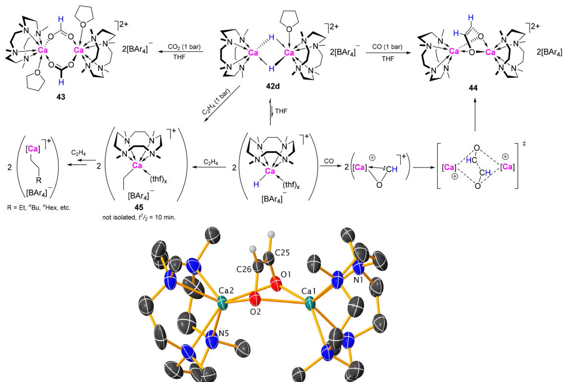
Scheme 15 Reactivity of compound 42d towards small molecules, and molecular structure of cis -enediolate 44 . Ar = C 6 H 3 -3,5-Me 2 .
