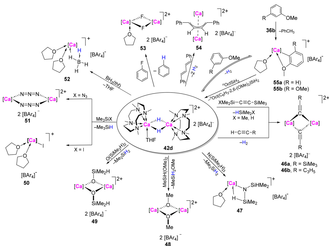
Scheme 16 Reactivity of calcium hydride 42d . [\text{Ca}] = [(\text{Me}_4\text{TACD})\text{Ca}]^{2+} ; Ar = C 6 H 3 -3,5-Me 2 .
