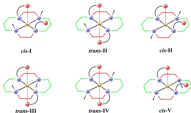
Fig. 1 Schematic representation and classification of the isomers of the \text{Cu}^{\text{II}} complexes with the cyclam ligands bearing two coordinating pendant arms. The isomers are labelled cis and trans according to the mutual position of the two pendant arms with respect to the macrocycle plane. trans isomers are typically hexacoordinated with a distorted octahedral coordination sphere, whereas cis isomers are pentacoordinated in a tetragonal pyramid.
