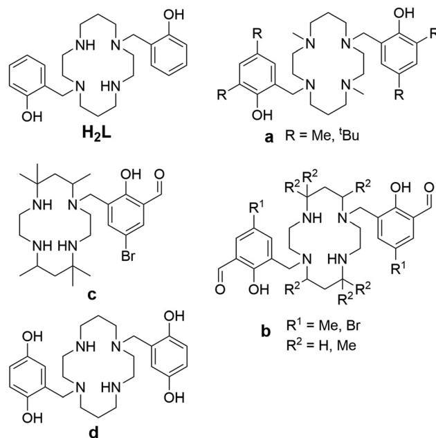
Fig. 2 The studied ligand \text{H}_2\text{L} and other previously reported cyclam-based ligands featuring phenolic pendant arms ( a – d ).
