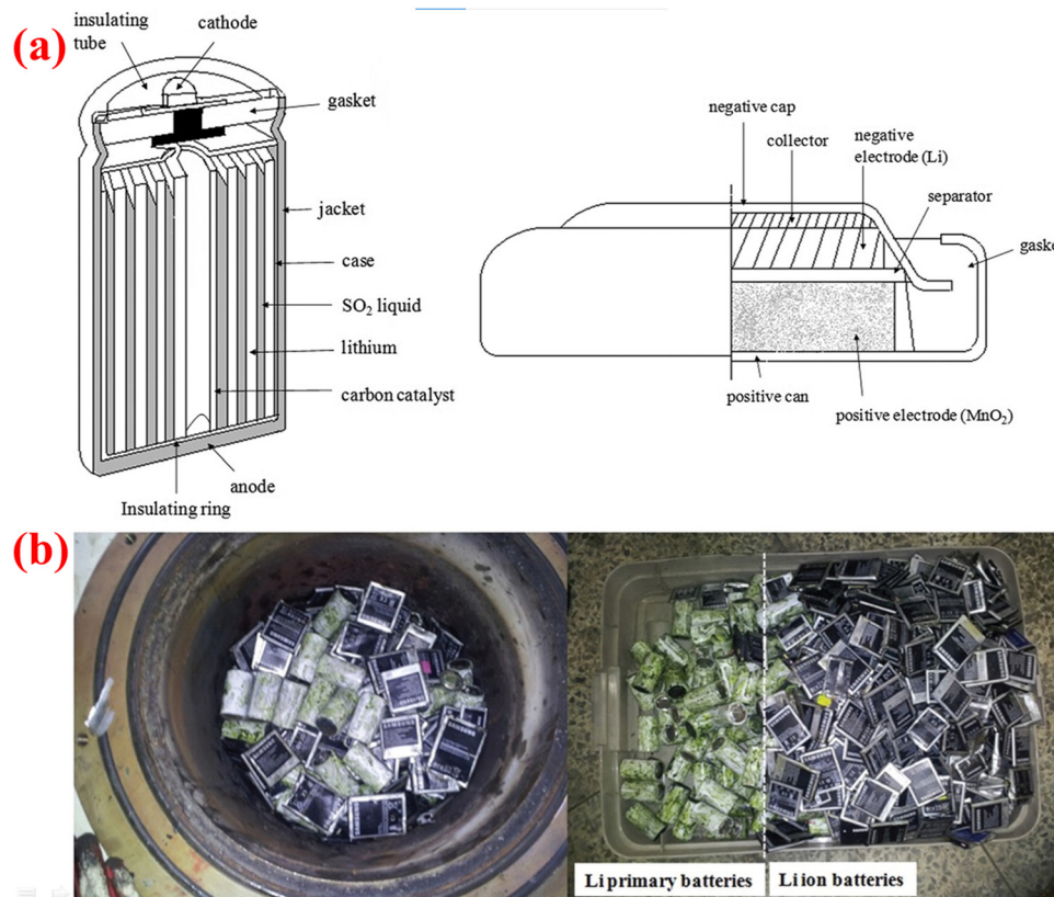
Fig. 5 (a) Schematic illustration of two types of lithium primary batteries: lithium sulfur dioxide ( \text{Li-SO}_2 ) and lithium manganese dioxide ( \text{Li-MnO}_2 ); (b) disposed lithium primary batteries (Li-primary) and lithium-ion (Li-ion) batteries in a recycling facility reproduced from ref. 56 copyright © IMechE 2015.
