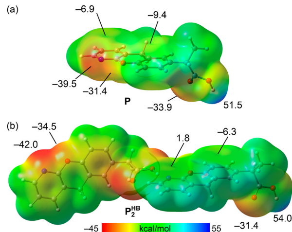
Fig. 5 MEP surface analysis of P (a) and \text{P}_2^{\text{HB}} (b). Selected surface energies are given in \text{kcal mol}^{-1} .
