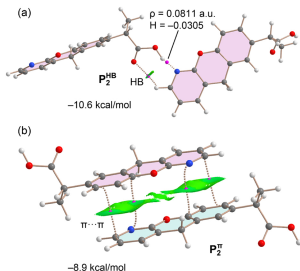
Fig. 6 Overlapped QTAIM and NCIplot analyses of the \text{P}_2^{\text{HB}} (a) and \text{P}_2^{\pi} (b) dimers. The dimerization energies are indicated. Bond critical points as fuchsia spheres and bond paths as dashed lines. Ring and cage critical points were omitted. For the NCIplot analysis, the following setting were used, S = 0.45 , \rho cut-off = 0.04 \text{ a.u.} , color scale -0.035 \leq \text{sign}(l_2)\rho \leq -0.035 \text{ a.u.} Only intermolecular interactions are represented.
