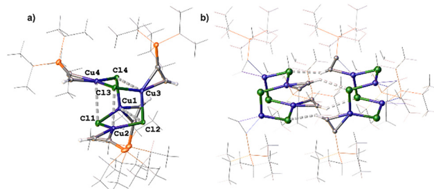
Fig. 2 Solid-state structure of ( 1 ). (a) The Cu 4 Cl 4 -core and SiCCH drawn as thermal ellipsoids (50% probability levels); i Pr-groups are rendered as wire frame for clarity. (b) Weak hydrogen bonding (CC-H...Cl) linking clusters of 1 into a 1D-network.
