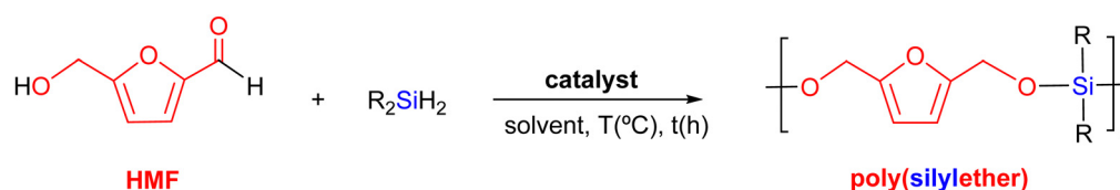
Scheme 7 Preparation of linear poly(silylethers) via copolymerisation of 5-hydroxymethyl furfural with dihydrosilanes and subsequent reaction with 1,4-diaminobutane.
