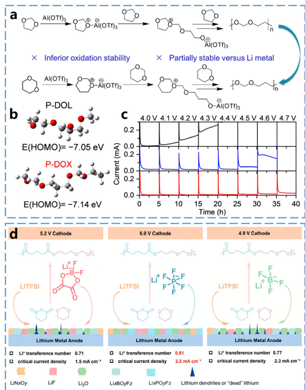
Fig. 6 In situ curing mechanisms of DOL and DOX polymerization processes initiated by \text{Al}(\text{OTf})_3 . (b) HOMO energies of P-DOL and P-DOX polymer chains. (c) Electrochemical float test of electrolyte in \text{Li}||\text{NCM111} battery. Reproduced from ref. 38 with permission from the Royal Society of Chemistry, copyright 2023. (d) Schematic illustration of the fabrication of PEA-PEs and the effect of salts on the compositions of SEI layers. Reproduced from ref. 39 with permission from John Wiley and Sons, copyright 2024.
