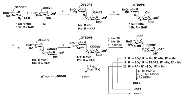
Scheme 1 Synthesis of glucuronic acid based HS disaccharides: (a) NIS, TMSOTf, DCM, -78^\circ\text{C} , 15 min; (b) thiourea, Py: MeOH (1: 1), 80^\circ\text{C} , 2 h; (c) (i) TEMPO, BAIB, DCM: H 2 O (1: 1), RT; (ii) MeI, K 2 CO 3 , DMF, 6 h, RT; (d) Zn dust, THF: AcOH: Ac 2 O (3: 2: 1), RT, 12 h; (e) HF.Py, Py, 0^\circ\text{C} , 12 h; (f) DDQ, DCM: H 2 O (18: 1), RT, 1 h; (g) LiOH, H 2 O: THF (1: 1), RT, 12 h; (h) BnBr, NaHCO 3 , DMF, 60^\circ\text{C} , 2 h; (i) SO 3 .Et 3 N, DMF, 60^\circ\text{C} , 48–72 h; and (j) H 2 , Pd(OH) 2 , H 2 O, RT, 48 h.
