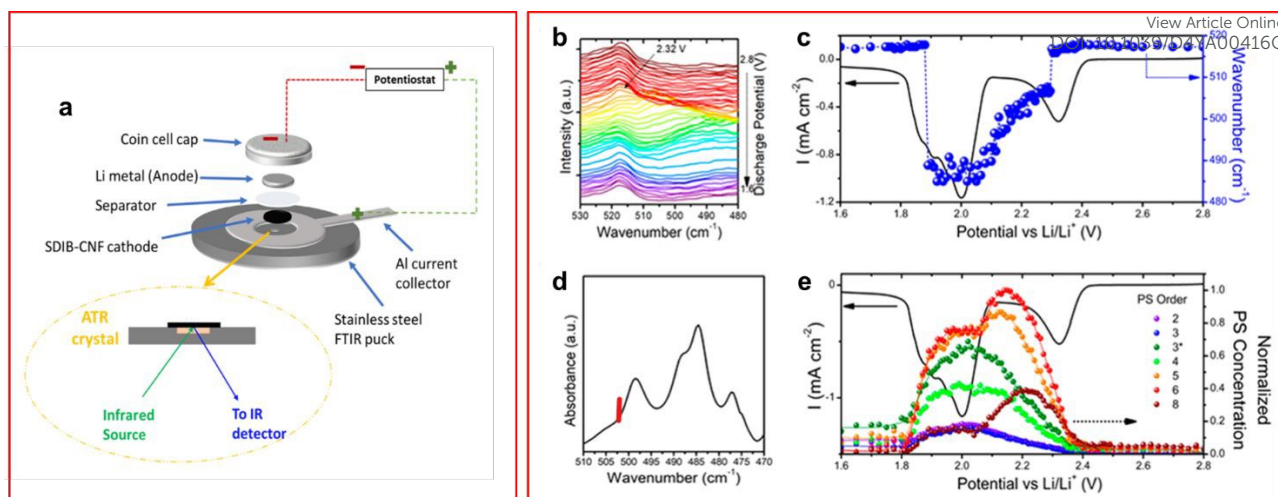
Fig. 4 (a) Schematic of ATR-IR cell configuration; (b) IR spectra obtained during a CV at a scan rate of 0.05 mV s -1 ; (c) CV of operando cell overlapped with spectral data from the most intense spectrum; (d) Single IR spectrum of the same cell at 2.2 V where multiple peaks assigned to LiPS species; (e) Deconvoluted peaks give individual LiPS species and hence concentration. The LiPS concentrations are shown to vary during discharge giving insight into the mechanism of discharge. ((a) Reproduced with permission from ref. 62, Copyright (2022) American Chemical Society; (b-e) Reproduced with permission from ref. 63, Copyright (2018) American Chemical Society).
