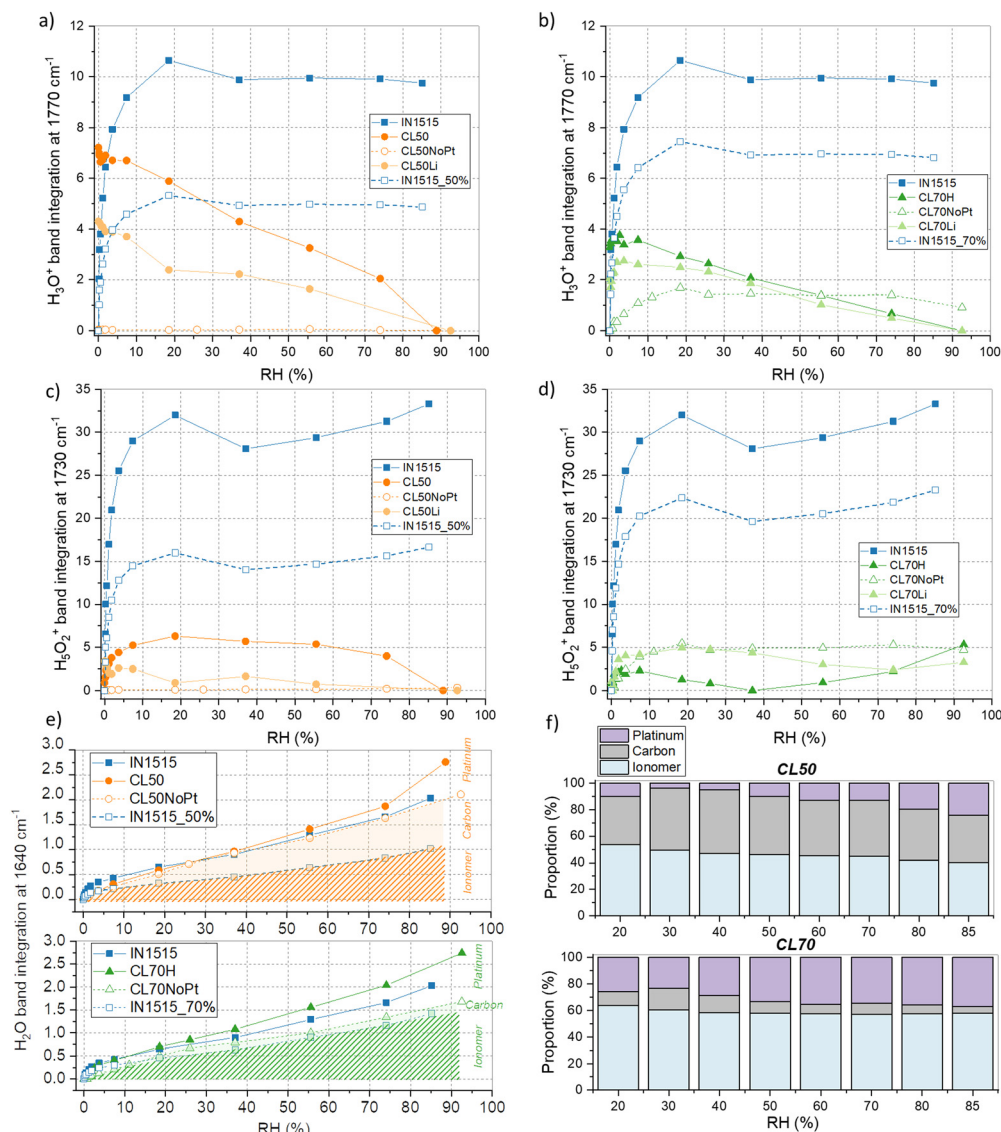
Fig. 7 Interactions of water with the ionomer, carbon, and platinum analyzed by IR. Band integration at 1770 , 1730 \text{cm}^{-1} (band normalized to ionomer backbone band at 1588 \text{cm}^{-1} , integration subtracted from its value at 0\% RH) versus humidity for (a), (c) CL50, CL50Li and CL50NoPt and (b), (d) CL70, CL70Li and CL70NoPt compared to the IN1515 membrane (IN1515_50% and IN1515_70% correspond to 50% and 70% of the integration values within these bands, respectively). (e) integration of bands at 1640 \text{cm}^{-1} versus humidity for (above) IN1515, CL50, CL50NoPt, and IN1515_50%, and (below) IN1515, CL70, CL70NoPt, and IN1515_70%, with indications of water proportions absorbed by ionomer, carbon, and platinum, (f) analytical simulation of water (corresponding to FTIR band at 1640 \text{cm}^{-1} ) in interaction with ionomer, carbon and platinum in CL50 and CL70.
