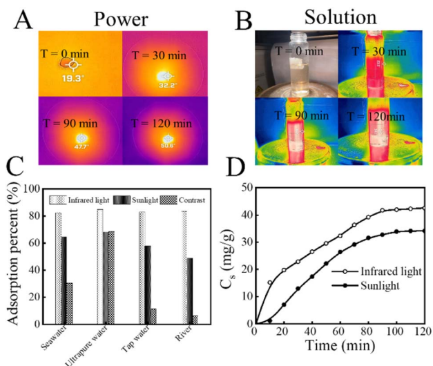
Fig. 6 Infrared images of KMnO_4@PAO powder (A) and 0.40 g per L KMnO_4@PAO suspension (B) under simulated sunlight irradiation; adsorption capability (C) and kinetics of KMnO_4@PAO for U(vi) under light irradiation (D). Light intensity: 0.20 \text{ W cm}^{-2} . T = 298 \text{ K} \pm 1 \text{ K} , contact time: 24 h, C[U(vi)]_{\text{initial}} = 20 \text{ mg L}^{-1} , m/V = 0.40 \text{ g L}^{-1} , pH = 8.2 \pm 0.1 , I = 0.1 \text{ mol per L NaCl} .
