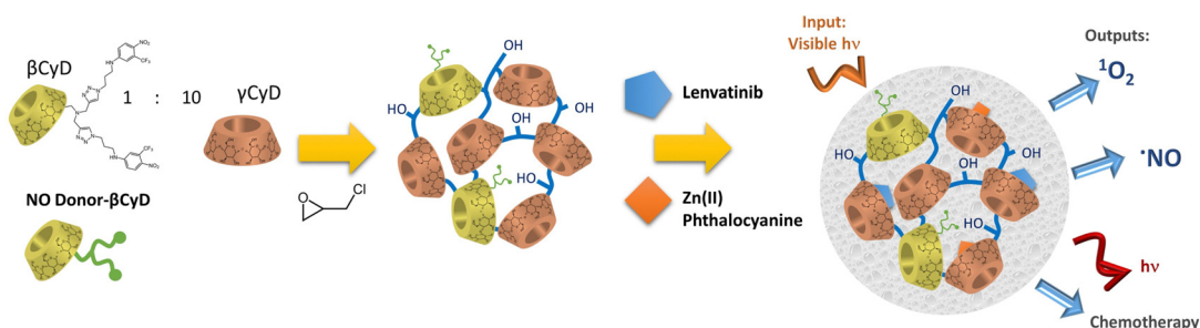
Fig. 5 Sketch of a NP achieved upon self-assembly of EPI-pβCyD, zinc phthalocyanine as red emitting ^1\text{O}_2 PS, lenvatinib as chemotherapeutic agent and the tailored molecular conjugate as green emitting NO donor.
