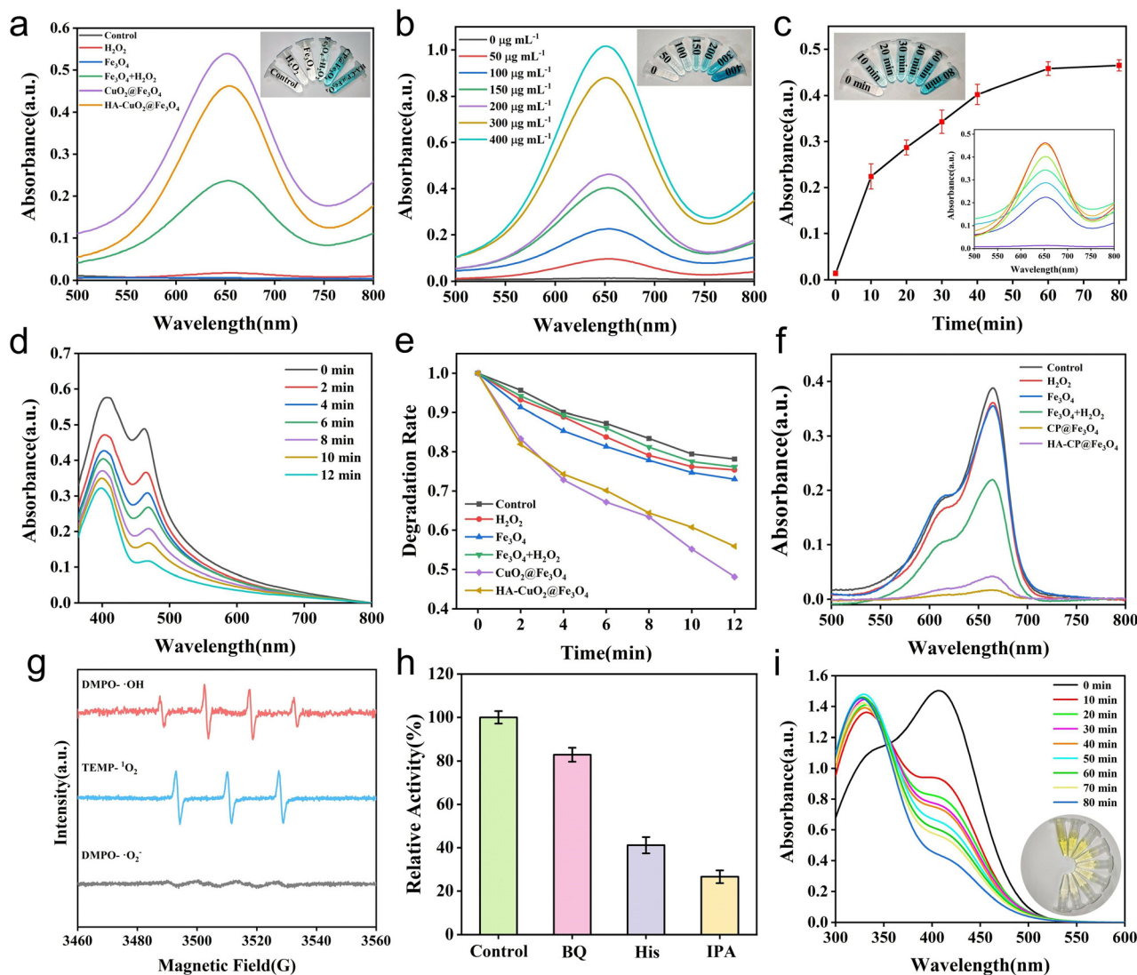
Fig. 3 (a) Confirmation of \bullet\text{OH} radicals generated by Fenton-like reaction in different groups ( 200 \mu\text{g mL}^{-1} ) using TMB assay. Studying Fenton activity of HA-CP@Fe 3 O 4 by varying (b) concentrations and (c) time ( 200 \mu\text{g mL}^{-1} ). (d) Absorption spectra of DPBF solution with HA-CP@Fe 3 O 4 ( 200 \mu\text{g mL}^{-1} ) at increasing time intervals. (e) Comparison of the degradation rates of DPBF over time in different experimental groups ( 200 \mu\text{g mL}^{-1} ). (f) Absorption spectra of MB after treatment with different experimental groups ( 200 \mu\text{g mL}^{-1} ). (g) ESR spin-trapping spectra of HA-CP@Fe 3 O 4 for the detection of DMPO- \bullet\text{OH} , DMPO- \bullet\text{O}_2^- , and TEMP- ^1\text{O}_2 . (h) Inhibition of TMB oxidation by IPA, BQ, and His in the presence of HA-CP@Fe 3 O 4 . (i) Time-dependent depletion of GSH by HA-CP@Fe 3 O 4 ( 200 \mu\text{g mL}^{-1} ).
