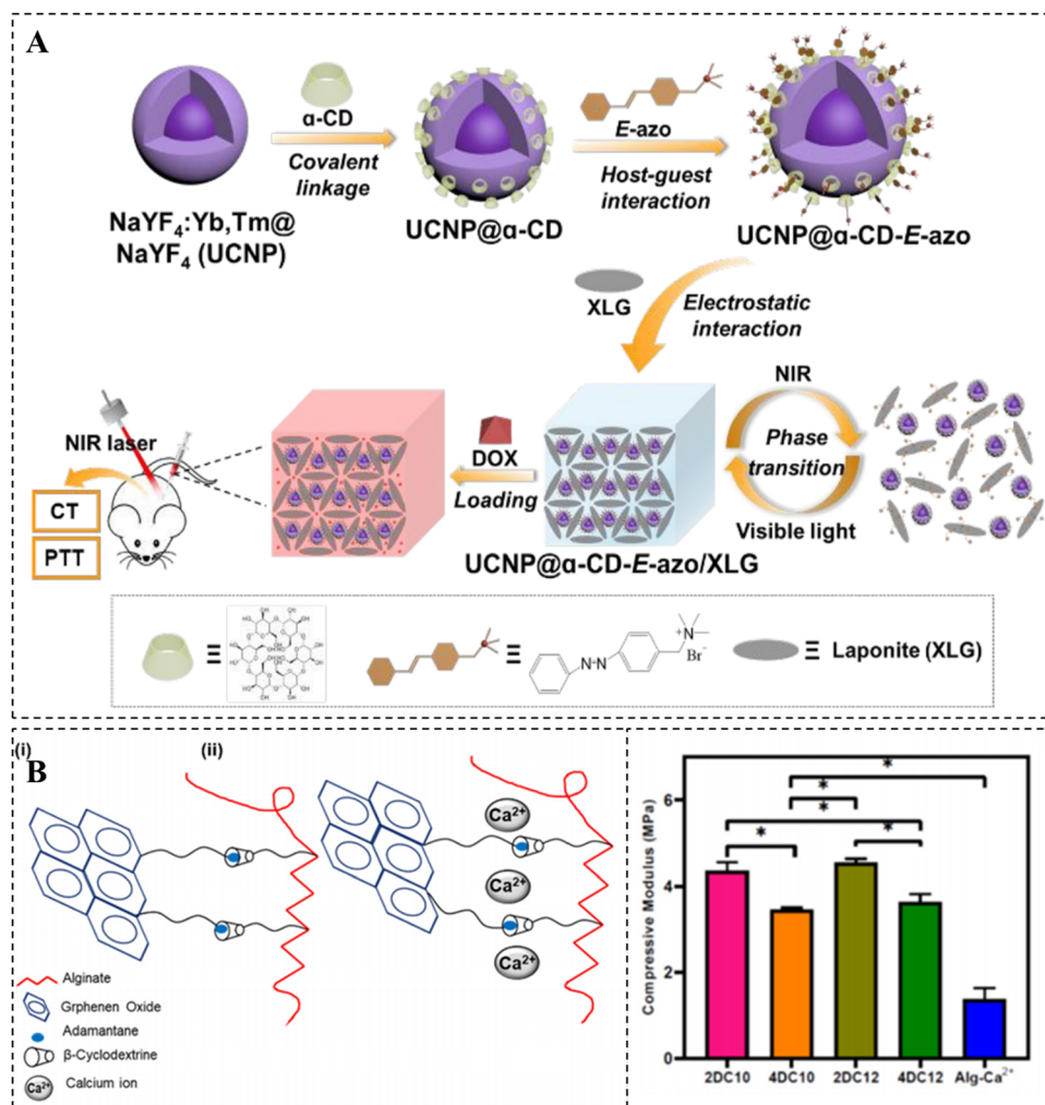
Fig. 3 Construction of CD-based supramolecular hydrogels based on ionic interactions. (A) NIR-responsive hydrogel via electrostatic interaction between UCNPs@α-CD-E-azo and LAPONITE ® and its pH/NIR-responsive DOX release. Reproduced with permission from ref. 95. Copyright 2020, Royal Society of Chemistry. (B) Crosslinking mechanism of the nanohybrid Alg-GO hydrogel with adjustable mechanical properties. Reproduced with permission from ref. 96. Copyright 2021, Elsevier.
