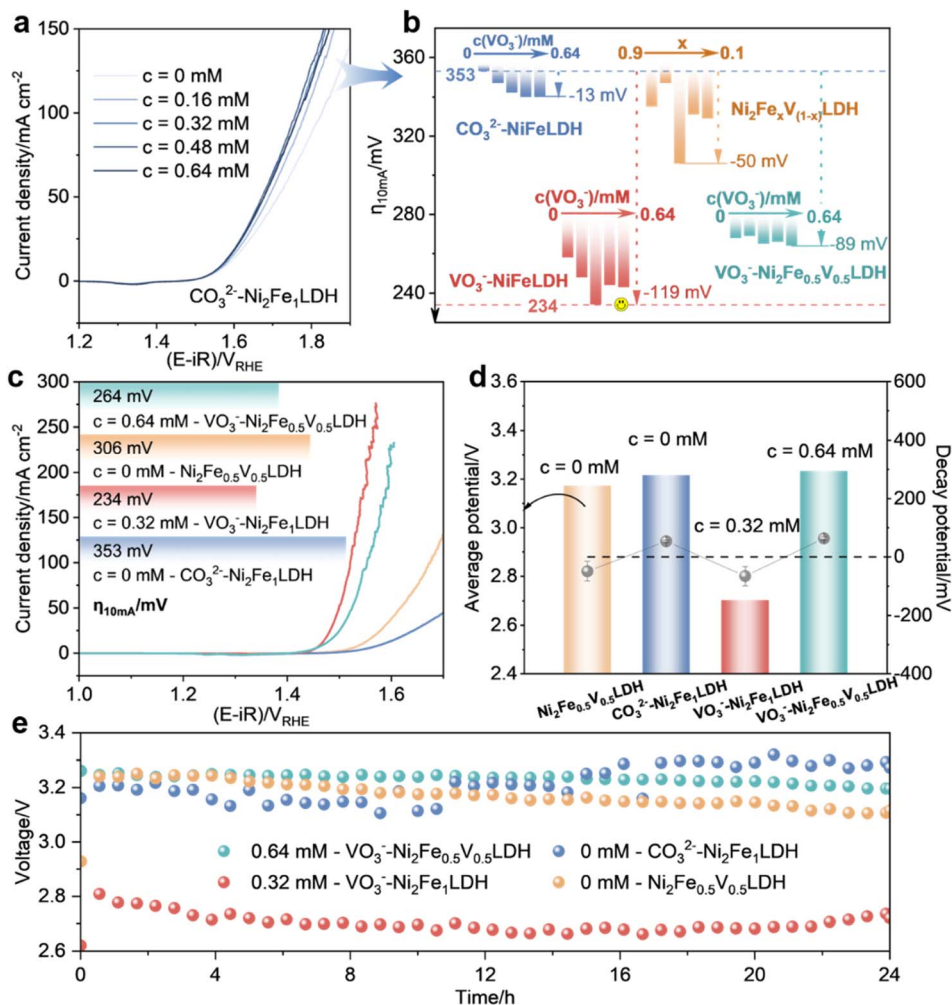
Fig. 2 (a) Cyclic voltammetry (CV) curve of CO 3 2- -Ni 2 Fe 1 LDHs in 1 M KOH + c mM NaVO 3 , respectively, scan rate of CV is 5 mV s -1 , (b) summary chart of overpotentials at 10 mA cm -2 of CO 3 2- -Ni 2 Fe 1 LDHs-catalyzed OER in 1 M KOH + c mM NaVO 3 (blue line), VO 3 - -Ni 2 Fe 1 LDHs-catalyzed OER in 1 M KOH + c mM NaVO 3 (red line), Ni 2 Fe x V (1-x) LDHs-catalyzed OER in 1 M KOH (yellow line), VO 3 - -Ni 2 Fe 0.5 V 0.5 LDHs-catalyzed OER in 1 M KOH + c mM NaVO 3 (green line), (c) LSV, (d) average voltage (bar graph) and decay voltage (point plot) data (with error bar) during the stability test of CO 3 2- -Ni 2 Fe 1 LDHs-catalyzed OER in 1 M KOH (blue line), VO 3 - -Ni 2 Fe 1 LDHs-catalyzed OER in 1 M KOH + 0.32 mM NaVO 3 (red line), Ni 2 Fe 0.5 V 0.5 LDHs-catalyzed OER in 1 M KOH (yellow line), VO 3 - -Ni 2 Fe 0.5 V 0.5 LDHs-catalyzed OER in 1 M KOH + 0.64 mM NaVO 3 (green line), (e) 24 h stability test data at 80 °C, 400 mA cm -2 in the two-electrode system.
