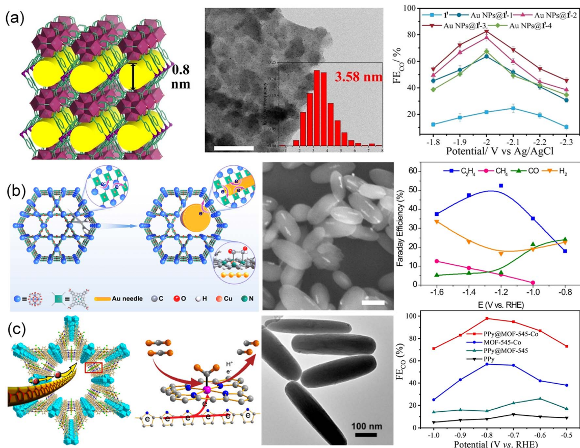
Fig. 7 (a) Three-dimensional framework of 1' , TEM image of Au-NPs@ 1'-3 and FE_{CO} of Au NPs@ 1'-x ( x = 1, 2, 3, \text{ and } 4 ). 51 Copyright 2022, Wiley-VCH. (b) Schematic illustration, the SEM image and FE for different products of the AuNN@PCN-222(Cu) catalyst. 188 Copyright 2022, Springer Nature. (c) Schematic illustration for the advantages of PPy in MOF-545-Co, the TEM image of PPy@MOF-545-Co and FE_{CO} of PPy@MOF-545-Co at different voltages. 189 Copyright 2021, American Chemical Society.
