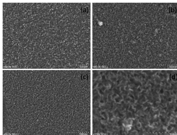
Fig. 3 SEM images of various samples grown at (a) 800\text{ }^{\circ}\text{C} on silicon (b) 800\text{ }^{\circ}\text{C} on quartz (c) and (d) 500\text{ }^{\circ}\text{C} on quartz.
