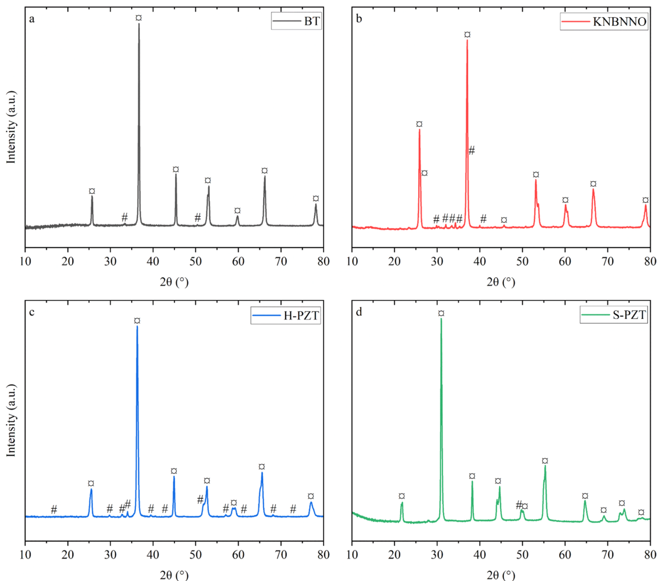
Fig. 1 XRD reflections of piezoceramic fillers: (a) BT, (b) KNBNNO, (c) H-PZT, and (d) S-PZT. Major perovskite phases are marked with 'ø' and secondary phases are marked with '#'.†
