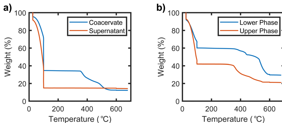
Fig. 3 TGA traces for (a) the coacervate and supernatant phases of a PSS − PDADMA + sample prepared below the binodal and (b) the dense and dilute phase of a sample prepared at a composition far above the binodal. The sample prepared under the binodal had a target composition of 3% PEC and 14% KBr by mass. The sample prepared in the upper phase window had a target composition of 20% PEC and 21% KBr by mass. TGA traces of all other samples prepared in both the UPW and the normal binodal regime exhibited similar trends (see ESI † ).
