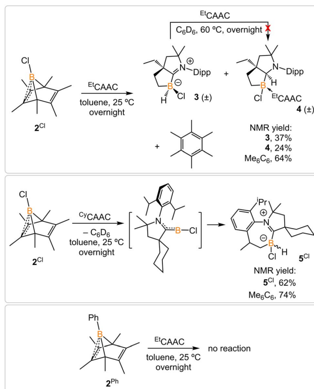
Scheme 2 Treatment of 2 Cl with \text{Et}^{\text{CAAC}} and \text{Cy}^{\text{CAAC}} and attempt to generate phenylborylene.
