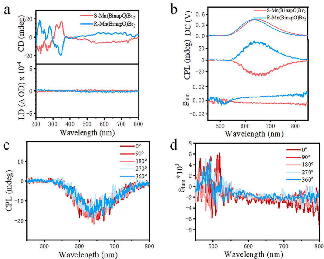
Fig. 2 (a) Circular dichroism absorption (CD) spectrum and linear dichroism absorption (LD) spectrum of R/S -Mn(Binapo)Br 2 . (b) Circularly polarized luminescence (CPL) spectra of (R/S) -Mn(Binapo)Br 2 with DC, CPL emission and g_{\text{lum}} . (c) CPL spectra of S -Mn(Binapo)Br 2 recorded by rotating the sample from 0^\circ to 360^\circ . (d) Variation of g_{\text{lum}} of S -Mn(Binapo)Br 2 measured after sample rotation from 0^\circ to 360^\circ .
