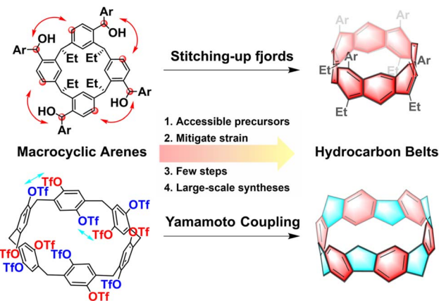
Fig. 1 Strategies and advantages for the synthesis of hydrocarbon belts using traditional macrocyclic arenes.
