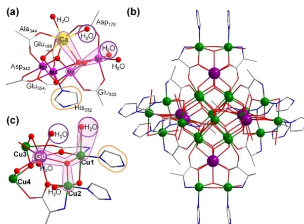
Fig. 1 (a) Structure of the \text{Mn}_4\text{CaO}_5 cluster. (b) Core of the \text{Gd}_6\text{Cu}_{24} -IM. (c) Asymmetric unit ( \text{GdCu}_4 ) of \text{Gd}_6\text{Cu}_{24} -IM. \text{H}_2\text{O}-\text{Ca}-\text{O}-\text{Mn}_2-\text{H}_2\text{O} and \text{H}_2\text{O}-\text{Gd}-\text{O}-\text{Cu}_2-\text{H}_2\text{O} motifs are marked in pink and water molecules are marked by a purple circle. Color codes: Gd, purple; Cu, green; Mn, pink; Ca, yellow; C, gray; N, blue; O, red. All H atoms were omitted.
