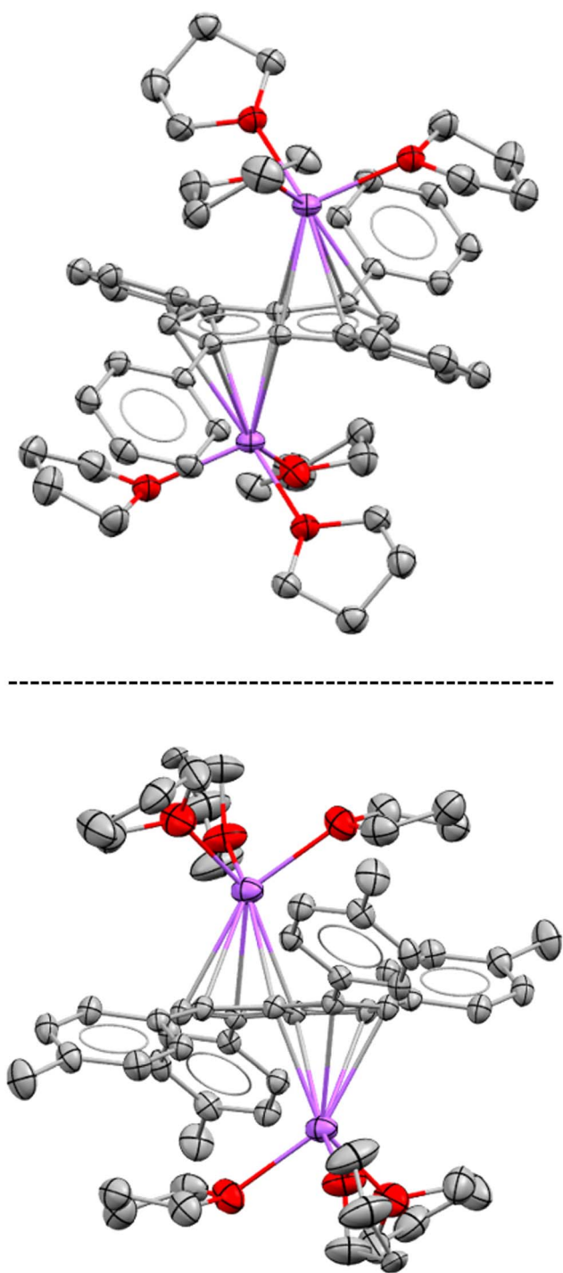
Fig. 1 XRD structures of [Na(THF)_3]_2[2] (top) and [Na(THF)_3]_2[3] (bottom) at 50% thermal probability with hydrogen atoms omitted for clarity (for details see the Experimental section).
