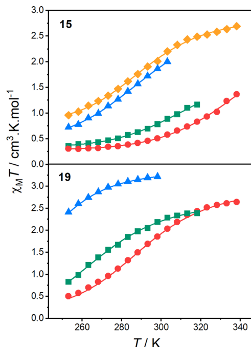
Fig. 6 Plots of \chi_M T vs. T obtained via Evans NMR method for solutions of 15 (top) and 19 (bottom) in DCE (orange \diamond ), DCM (blue \blacktriangle ), acetone (green \blacksquare ) and MeCN (red \bullet ). Respective solid lines indicate fits to the regular solution model.
