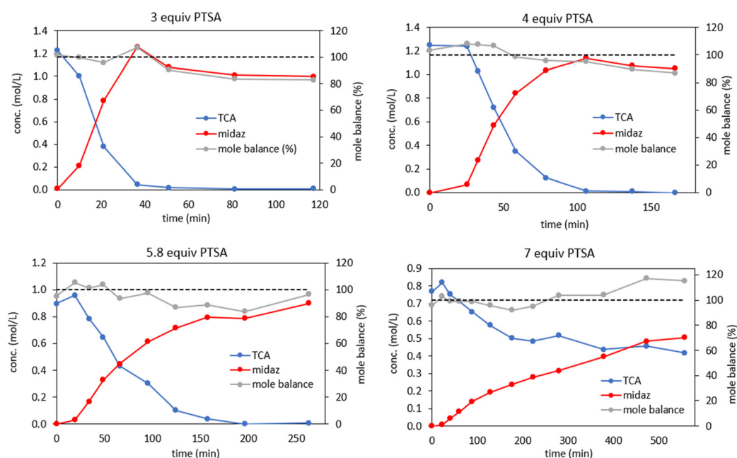
Fig. 1 Concentration profiles for small scale batch syntheses of midazolam from TCA using different equivalents of PTSA. All reactions were performed at 200 °C (midaz = midazolam). The lines are for illustrative purposes and are not intended to imply a modeled system. Mole balance is calculated by dividing the sum of the midazolam and TCA concentrations by the initial TCA concentration.
