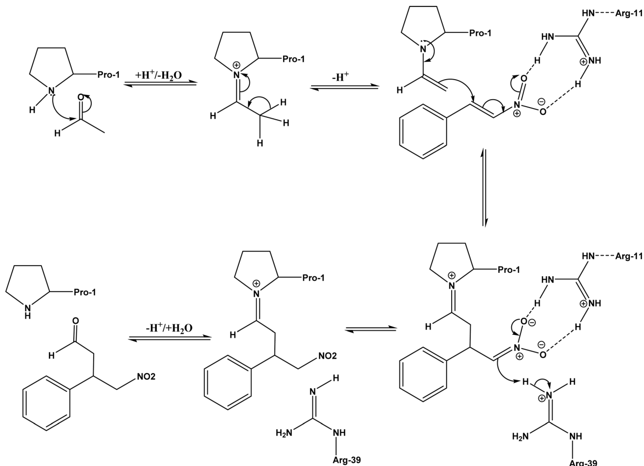
Fig. 40 Mechanism of Michael addition of trans -nitrostyrenes and acetaldehyde catalyzed by 4-oxalocrotonate tautomerase [redrawn from Scheme S1 in ref. 149].
