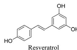
Resveratrol
