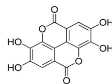
Ellagic Acid
