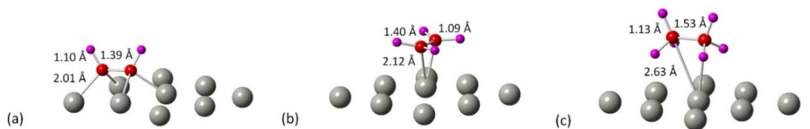
Pd 309 [111] Facet
