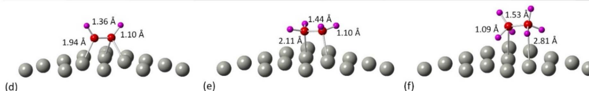
Fig. 4 The relaxed structures of (a) C 2 H 2 on the [100] facet of Pd 309 NP, (b) C 2 H 4 on the [100] facet of Pd 309 NP, (c) C 2 H 6 on the [100] facet of Pd 309 NP, (d) C 2 H 2 on the [111] facet of Pd 309 NP, (e) C 2 H 4 on the [111] facet of Pd 309 NP and (f) C 2 H 6 on the [111] facet of Pd 309 NP. Grey spheres represent Pd atoms, red spheres represent C atoms and purple spheres represent H atoms. Geometry relaxations were performed on the entire Pd NP–ligand complexes.
