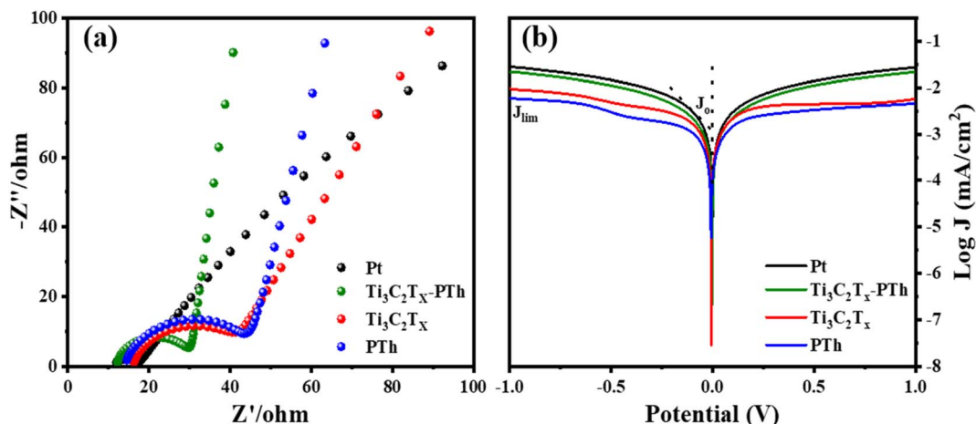
Fig. 7 (a) Electrochemical impedance spectra of Pt, \text{Ti}_3\text{C}_2\text{T}_x , PTh and \text{Ti}_3\text{C}_2\text{T}_x -PTh CE made from the symmetrical cell (b) Tafel polarisation of Pt, \text{Ti}_3\text{C}_2\text{T}_x , PTh and \text{Ti}_3\text{C}_2\text{T}_x -PTh CE.
