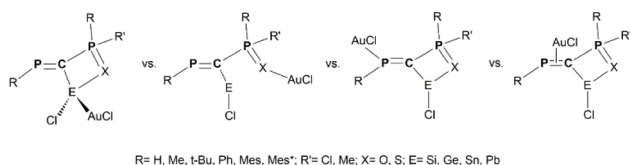
Scheme 3 Schematic representation of model \{\text{R}-\text{P}=\text{C}(\text{E}(\text{II}))(\text{Cl})-\text{P}(\text{X})\text{RR}'\}\text{AuCl} coordination isomers obtained via \text{E}(\text{II}) \rightarrow \text{Au} , \text{X} \rightarrow \text{Au} , \text{P}(\text{sp}^2) \rightarrow \text{Au} and \pi(\text{C}=\text{P}) \rightarrow \text{Au} bonds.
