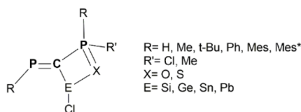
Scheme 2 General representation of the investigated \text{RP}=\text{C}(\text{E}(\text{II}))-\text{P}(\text{X})\text{RR}' model systems.
