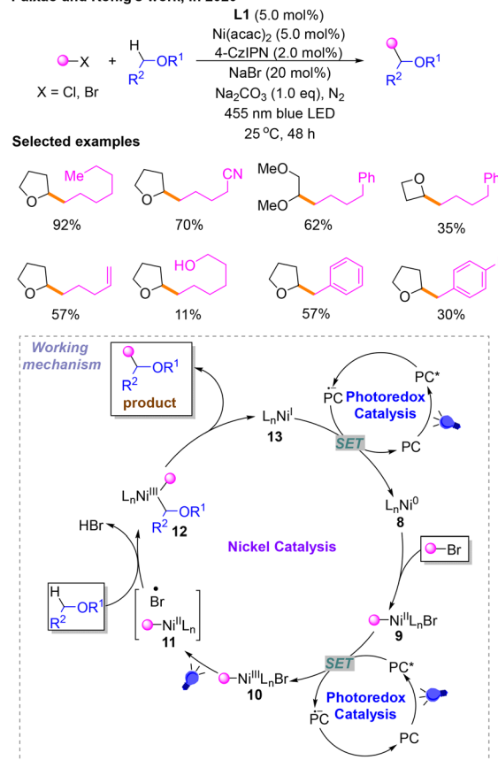
Scheme 5 Csp 3 –Csp 3 cross-coupling reaction of alkyl bromides with ethers (Paixão and Köniq’s work).
