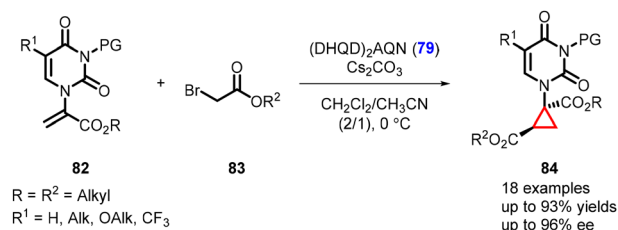
Scheme 15 Enantioselective cyclopropanation of α-pyrimidine substituted acrylates.
