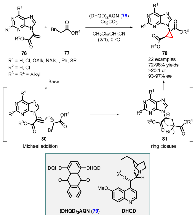
Scheme 14 Enantioselective cyclopropanation of α-purine acrylate.
